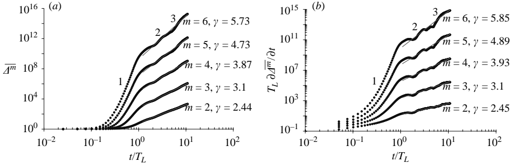
FIGURE 21. (a) \overline{\Delta}^m and its (b) time derivative versus time for various values of m (2, 3, 4, 5, 6). The straight lines correspond to power-law fittings with \overline{\Delta}^m \sim t^\gamma , the values of \gamma are given on the graph. (1 619 484 pairs.)
